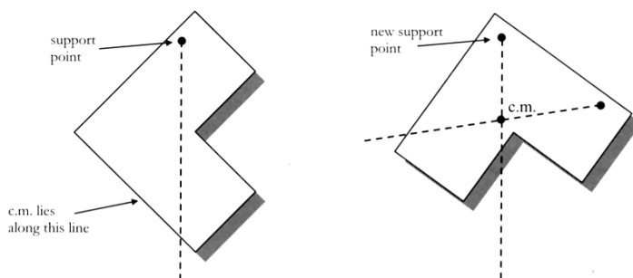
Figure 4.1 Finding centre of mass of a lamina
